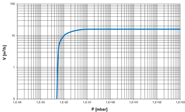
Pumping speed curve
